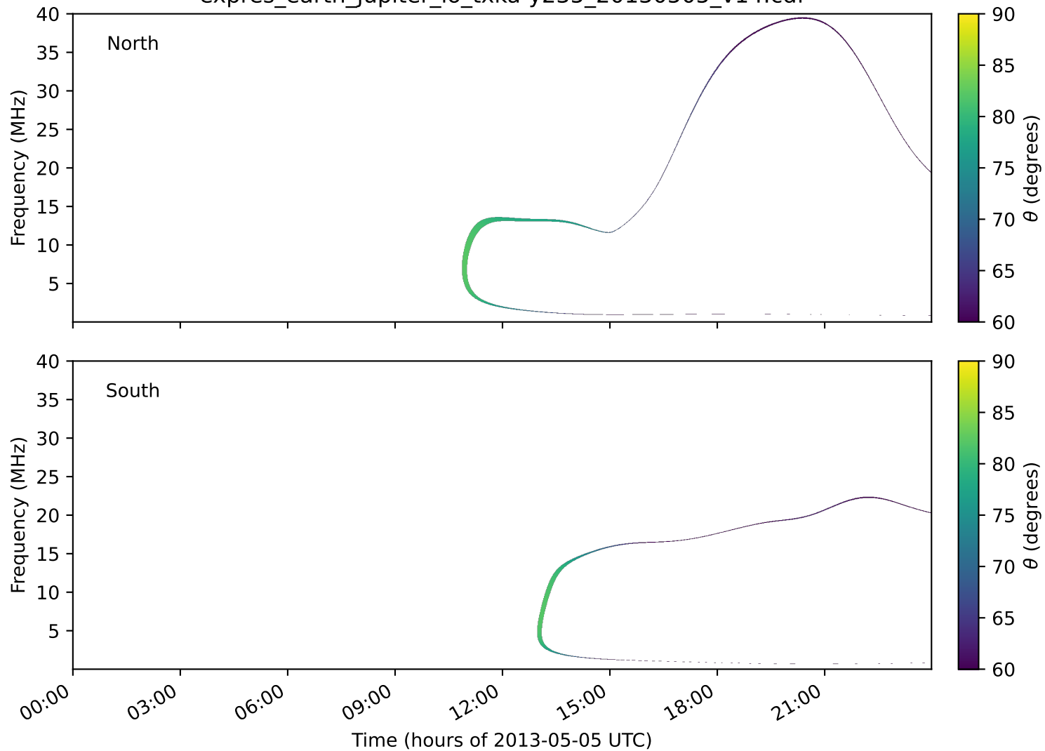
expres_earth_jupiter_io_txka-y235_20130505_v14.cdf
