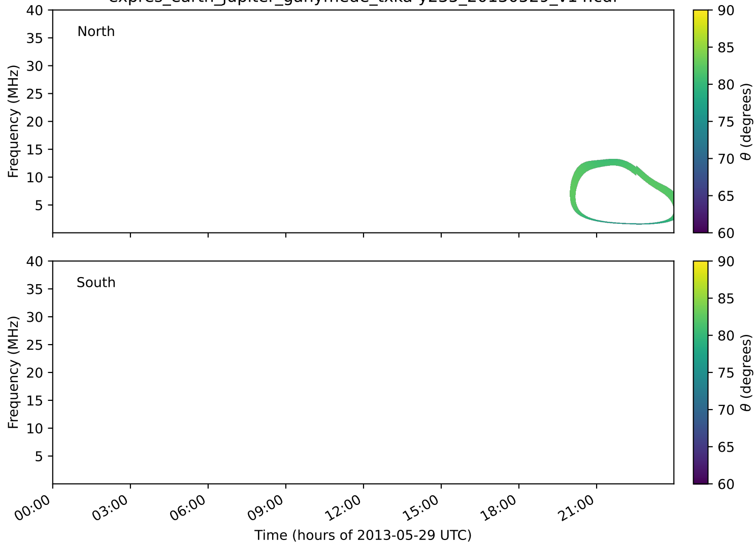
expres_earth_jupiter_ganymede_txka-y235_20130529_v14.cdf
