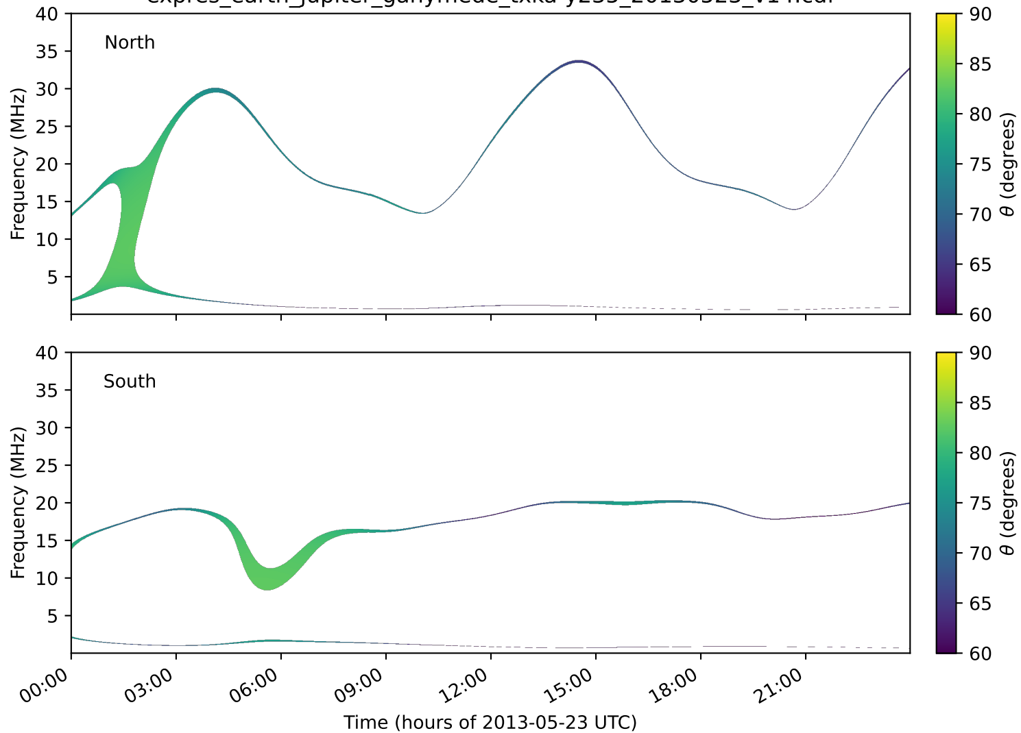
expres_earth_jupiter_ganymede_txka-y235_20130523_v14.cdf
