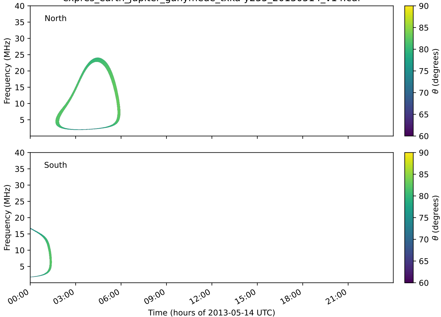
expres_earth_jupiter_ganymede_txka-y235_20130514_v14.cdf
