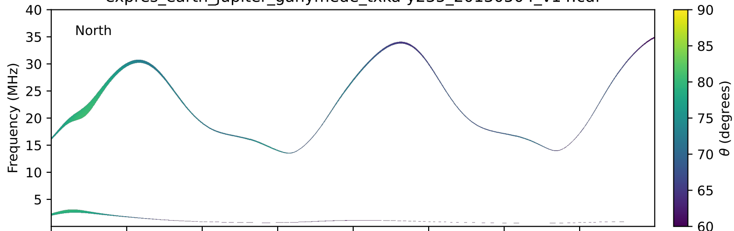
expres_earth_jupiter_ganymede_txka-y235_20130504_v14.cdf
