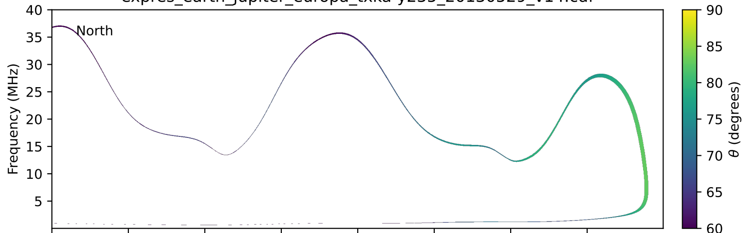
expres_earth_jupiter_europa_txka-y235_20130529_v14.cdf
