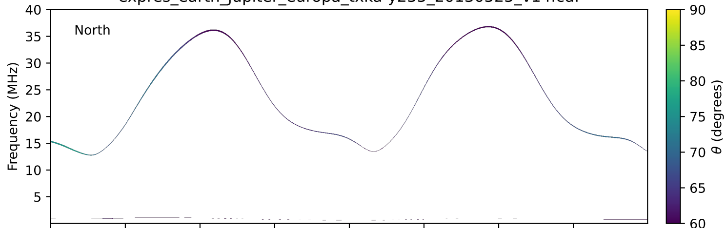
expres_earth_jupiter_europa_txka-y235_20130525_v14.cdf
