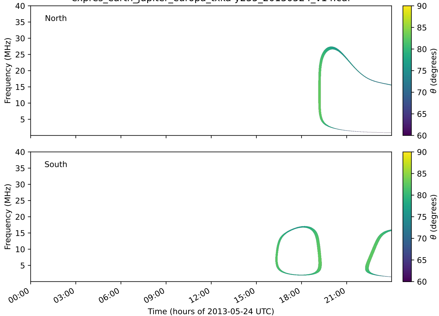
expres_earth_jupiter_europa_txka-y235_20130524_v14.cdf
