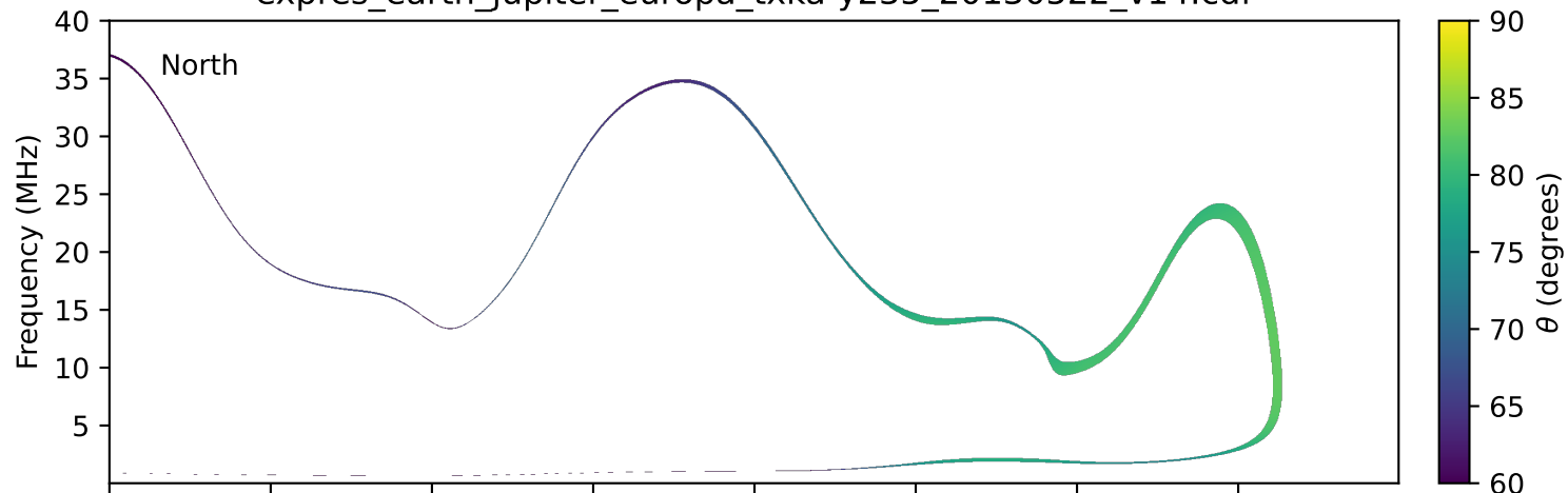
expres_earth_jupiter_europa_txka-y235_20130522_v14.cdf
