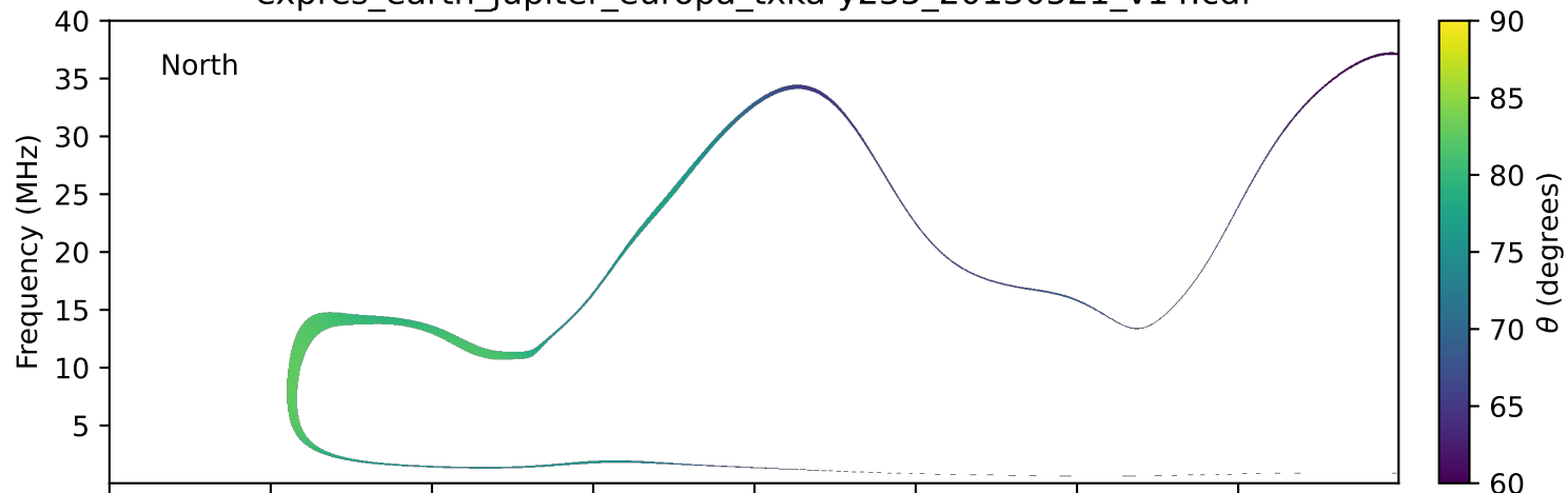
expres_earth_jupiter_europa_txka-y235_20130521_v14.cdf
