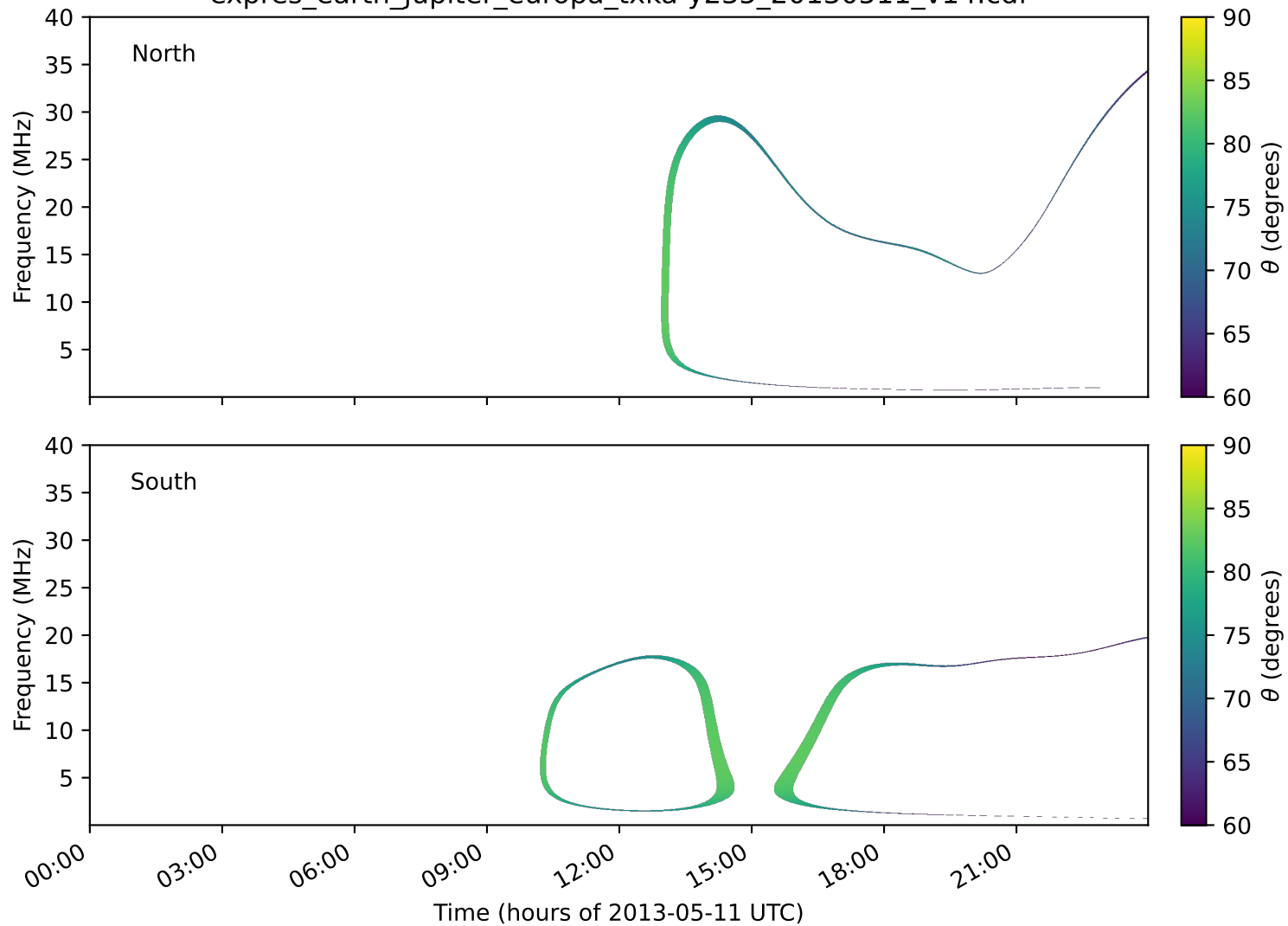
expres_earth_jupiter_europa_txka-y235_20130511_v14.cdf
