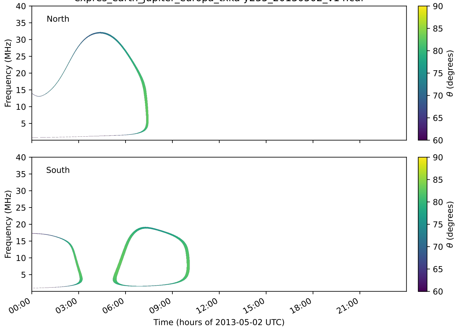
expres_earth_jupiter_europa_txka-y235_20130502_v14.cdf
