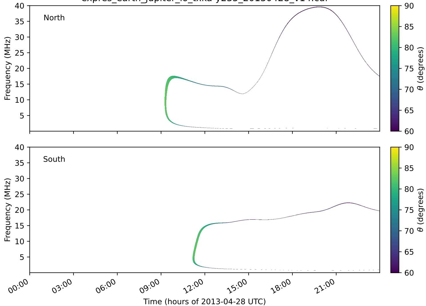
expres_earth_jupiter_io_txka-y235_20130428_v14.cdf
