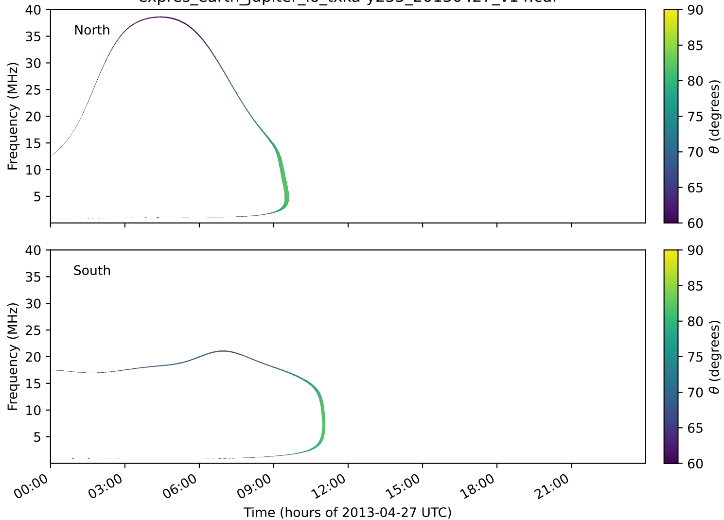
expres_earth_jupiter_io_txka-y235_20130427_v14.cdf
