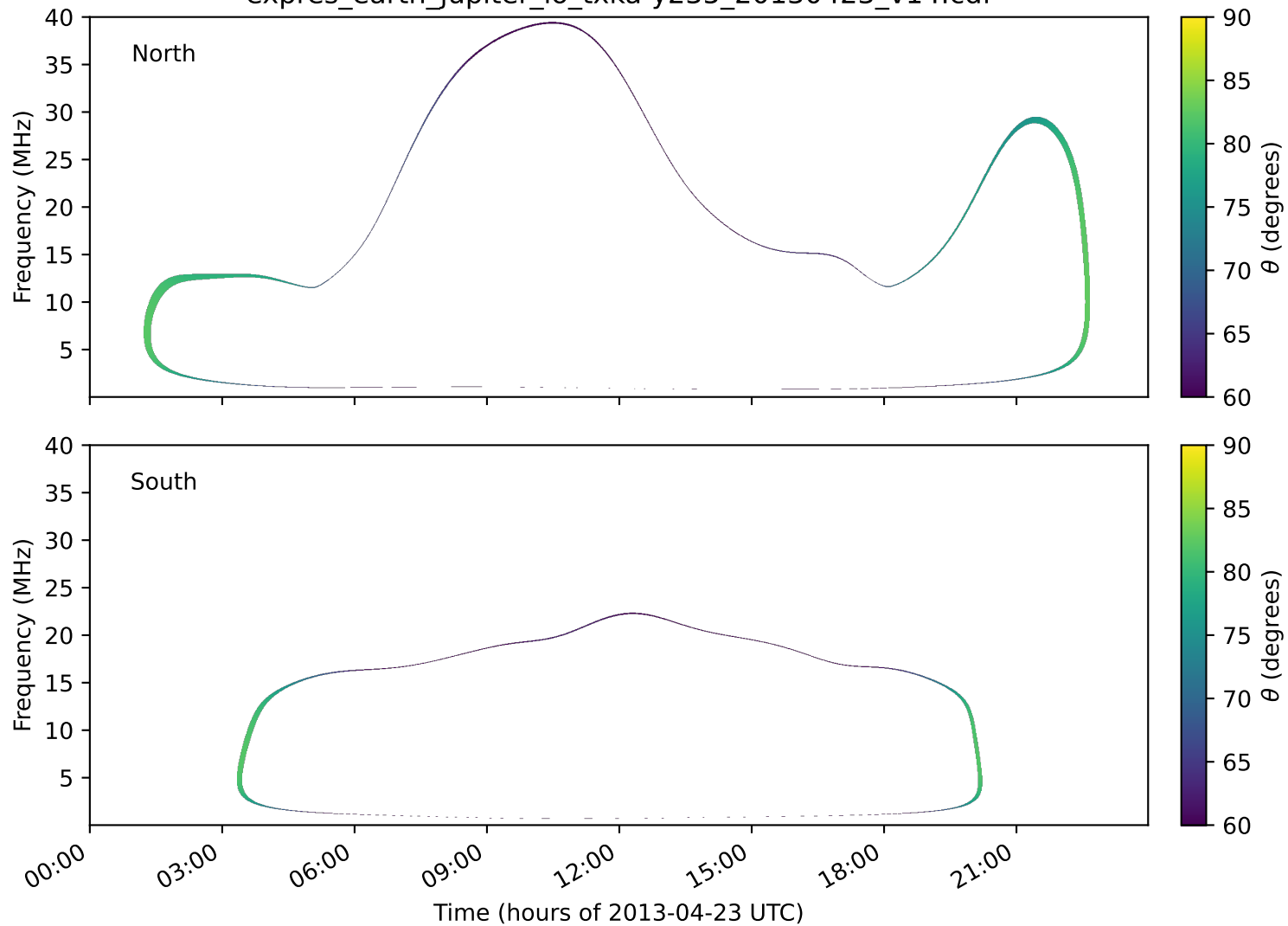
expres_earth_jupiter_io_txka-y235_20130423_v14.cdf
