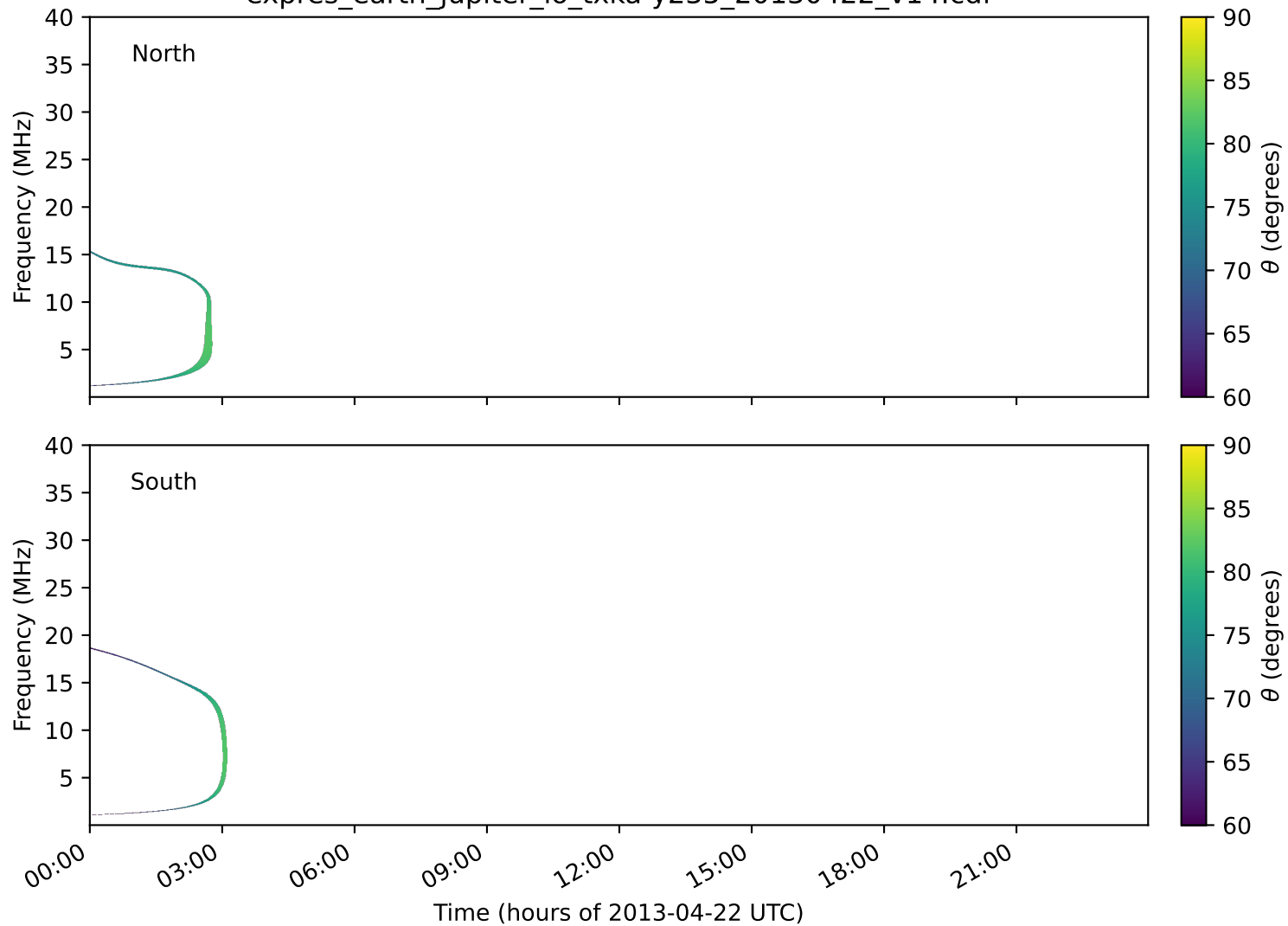
expres_earth_jupiter_io_txka-y235_20130422_v14.cdf
