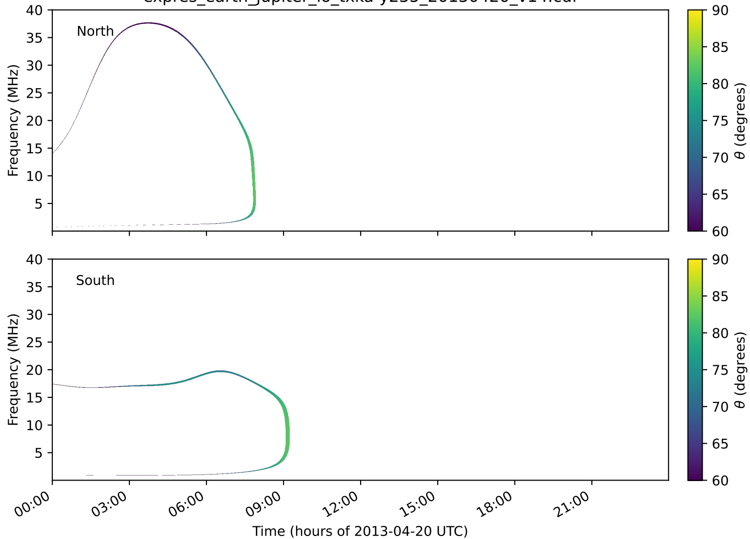
expres_earth_jupiter_io_txka-y235_20130420_v14.cdf
