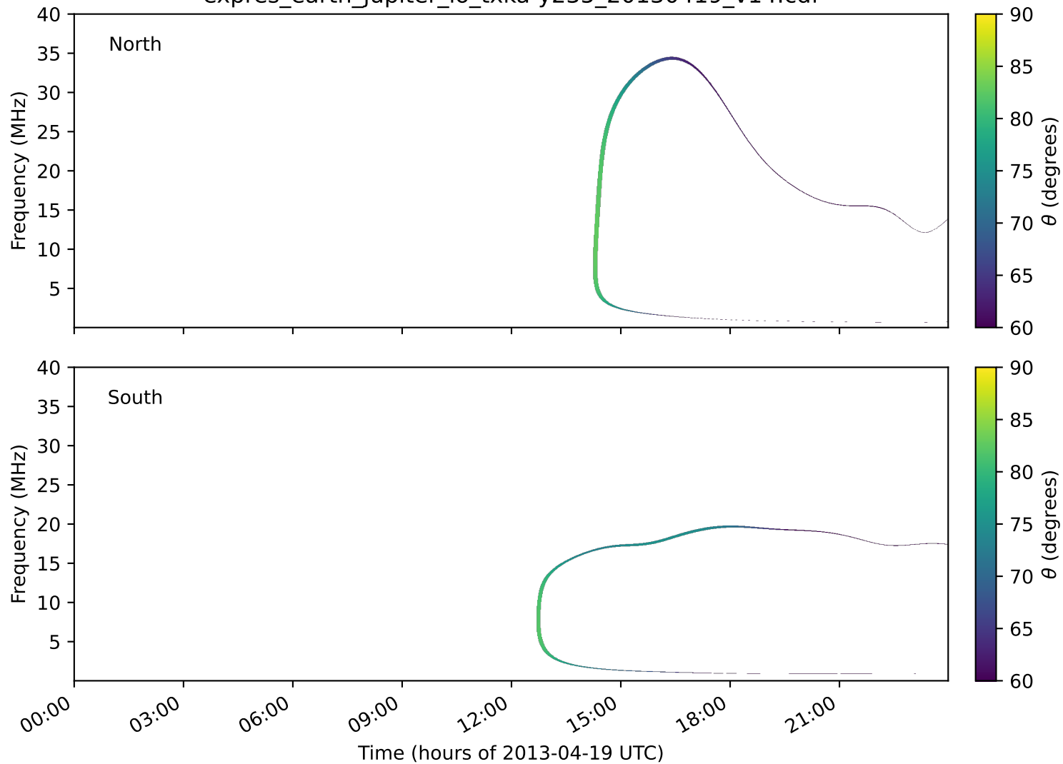
expres_earth_jupiter_io_txka-y235_20130419_v14.cdf
