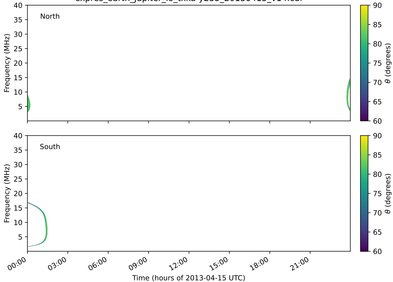
expres_earth_jupiter_io_txka-y235_20130415_v14.cdf
