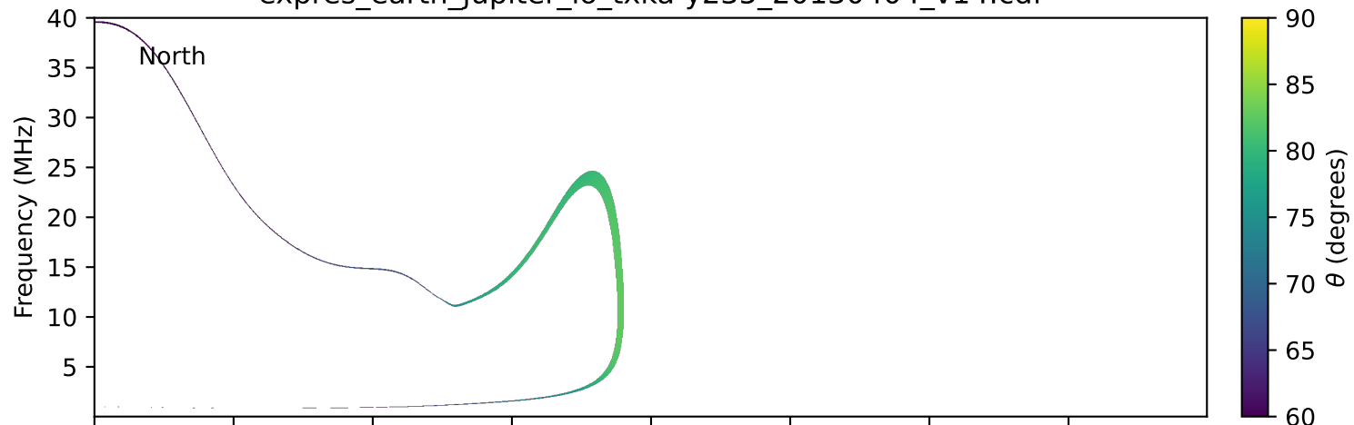
expres_earth_jupiter_io_txka-y235_20130404_v14.cdf
