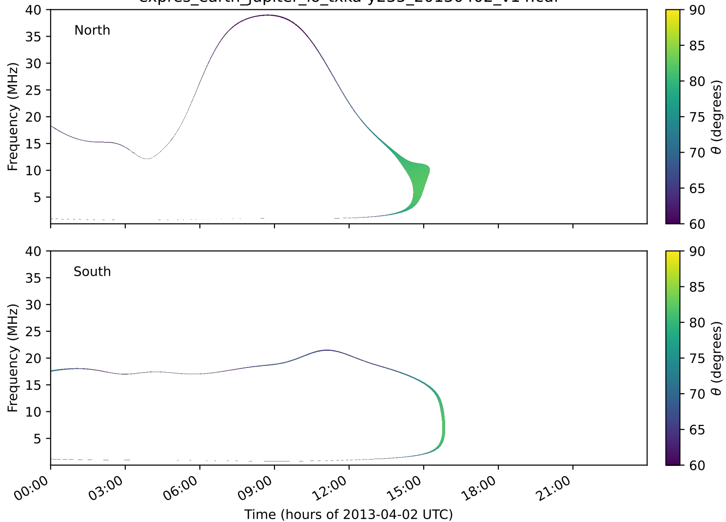
expres_earth_jupiter_io_txka-y235_20130402_v14.cdf
