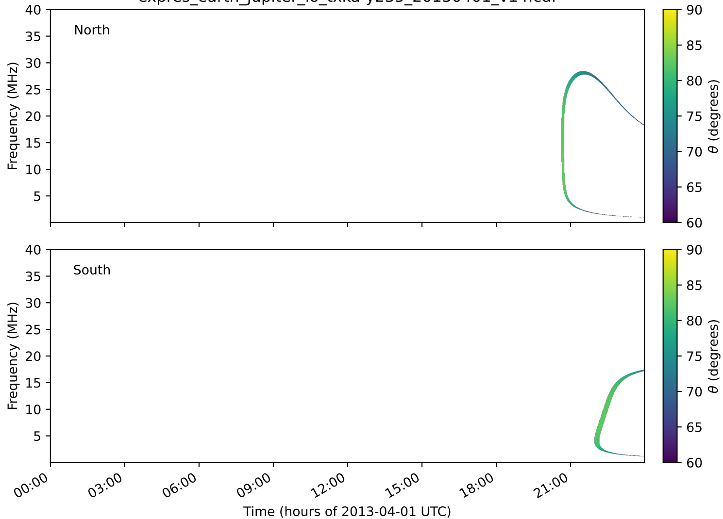
expres_earth_jupiter_io_txka-y235_20130401_v14.cdf
