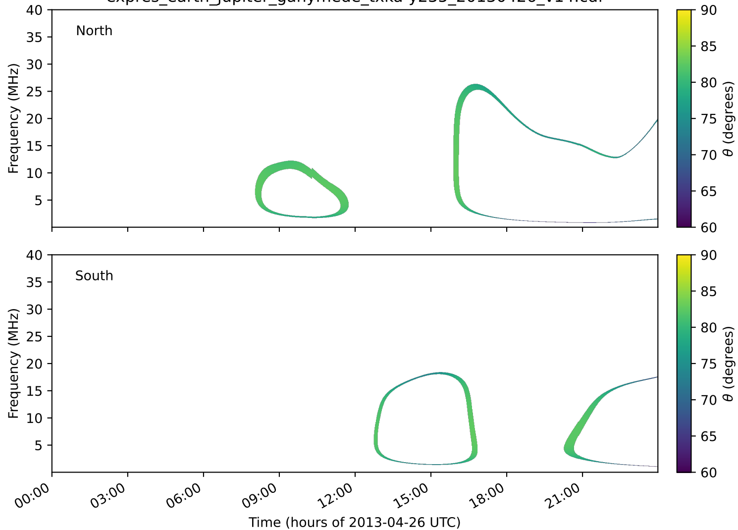
expres_earth_jupiter_ganymede_txka-y235_20130426_v14.cdf
