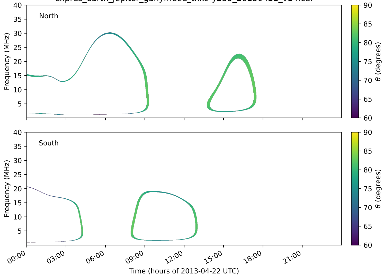
expres_earth_jupiter_ganymede_txka-y235_20130422_v14.cdf
