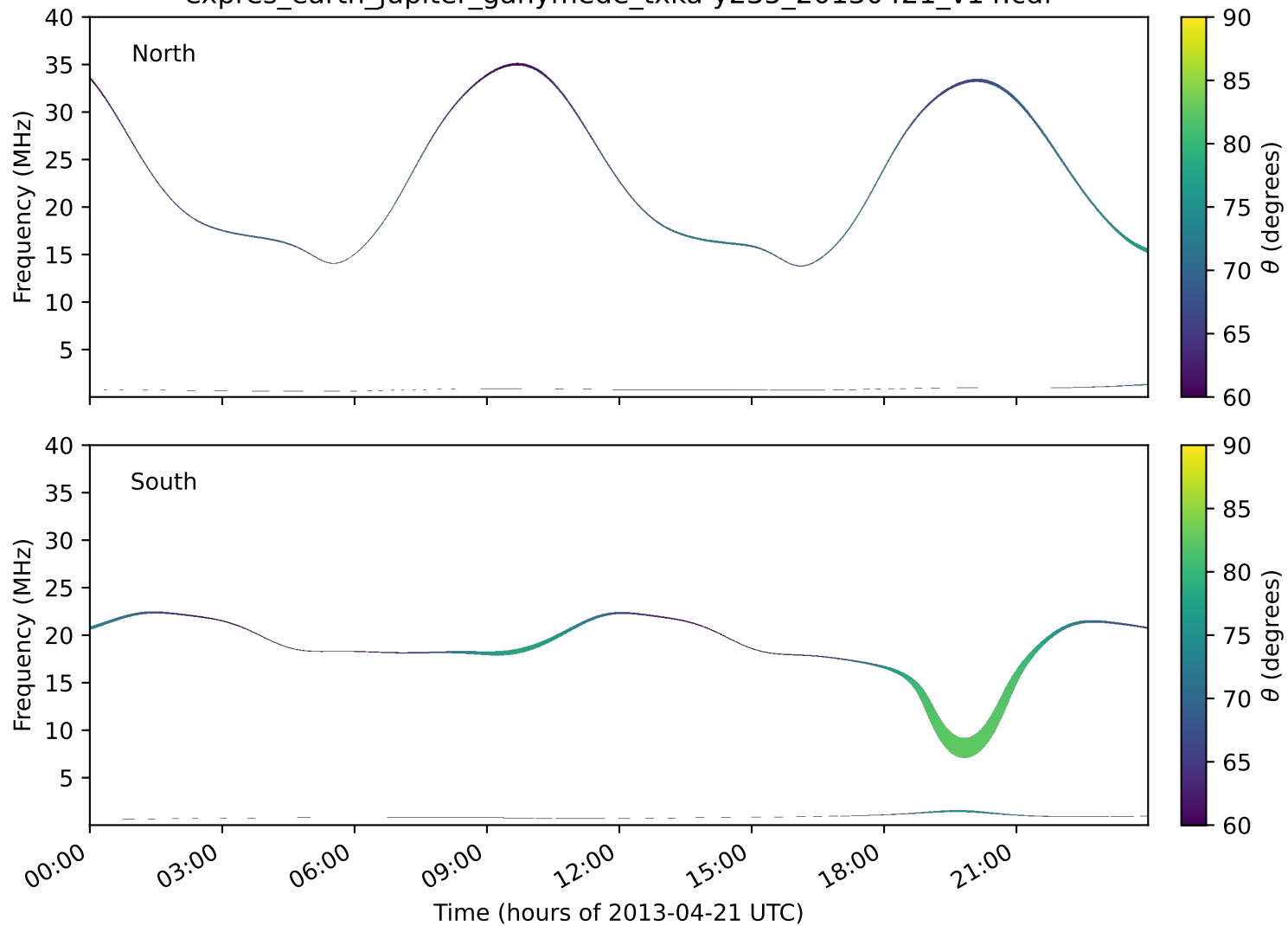
expres_earth_jupiter_ganymede_txka-y235_20130421_v14.cdf
