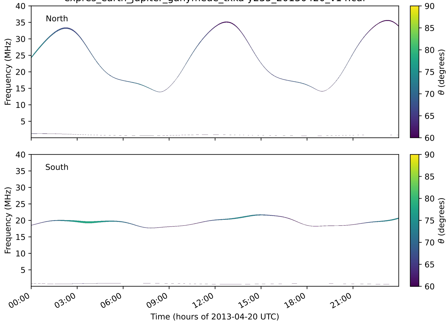
expres_earth_jupiter_ganymede_txka-y235_20130420_v14.cdf
