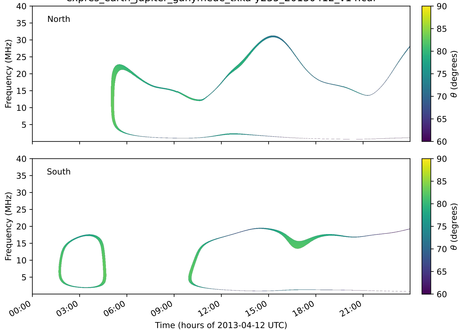
expres_earth_jupiter_ganymede_txka-y235_20130412_v14.cdf
