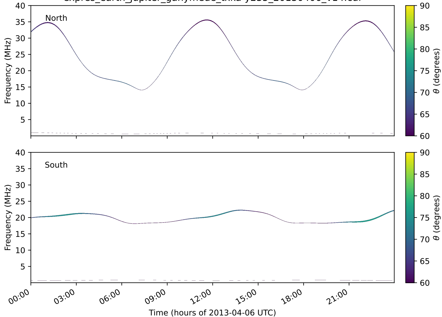
expres_earth_jupiter_ganymede_txka-y235_20130406_v14.cdf
