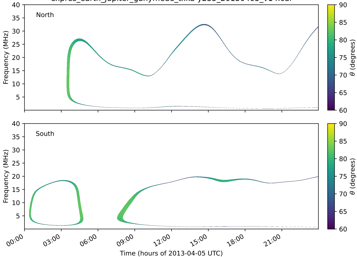
expres_earth_jupiter_ganymede_txka-y235_20130405_v14.cdf
