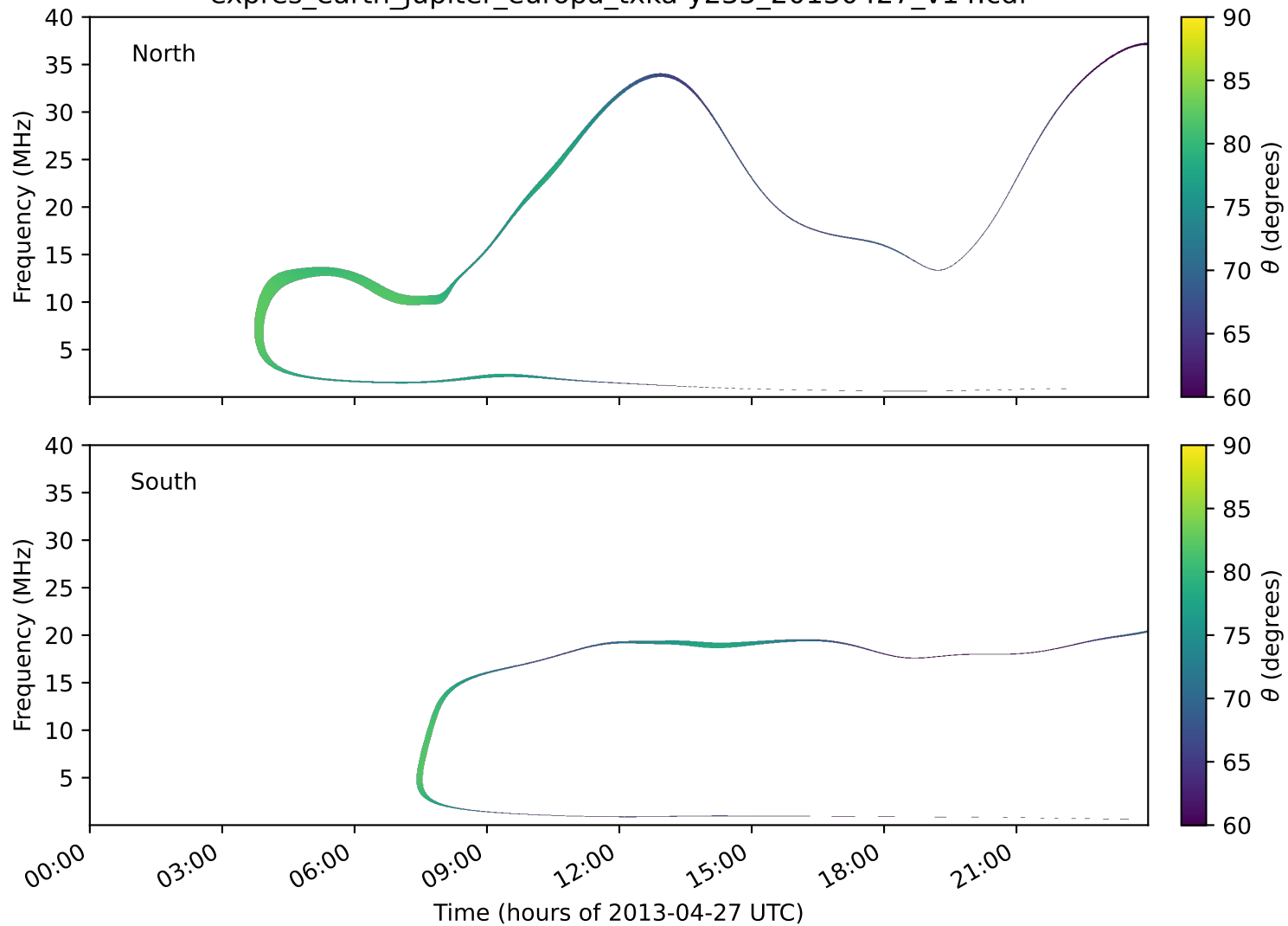
expres_earth_jupiter_europa_txka-y235_20130427_v14.cdf
