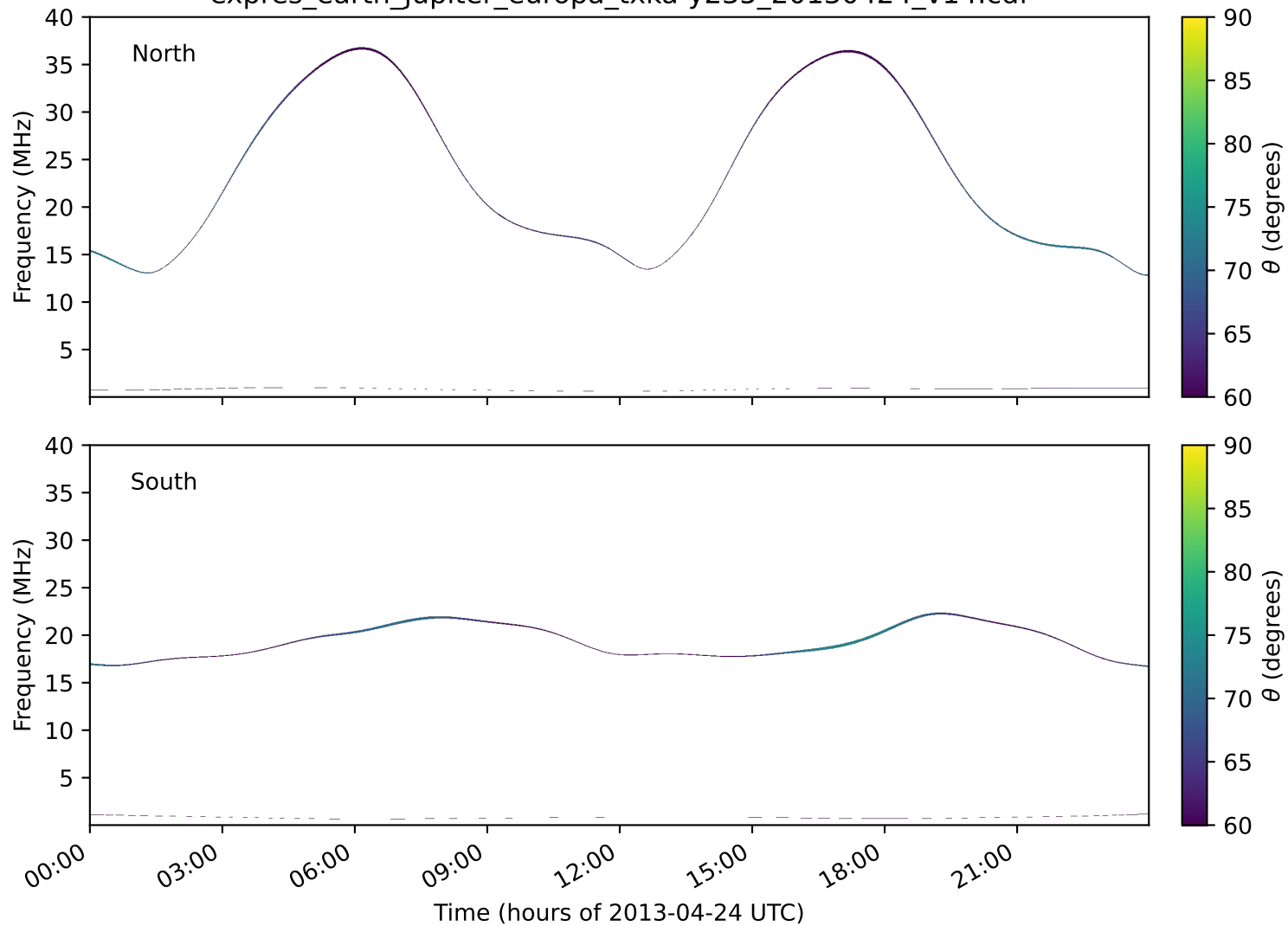
expres_earth_jupiter_europa_txka-y235_20130424_v14.cdf
