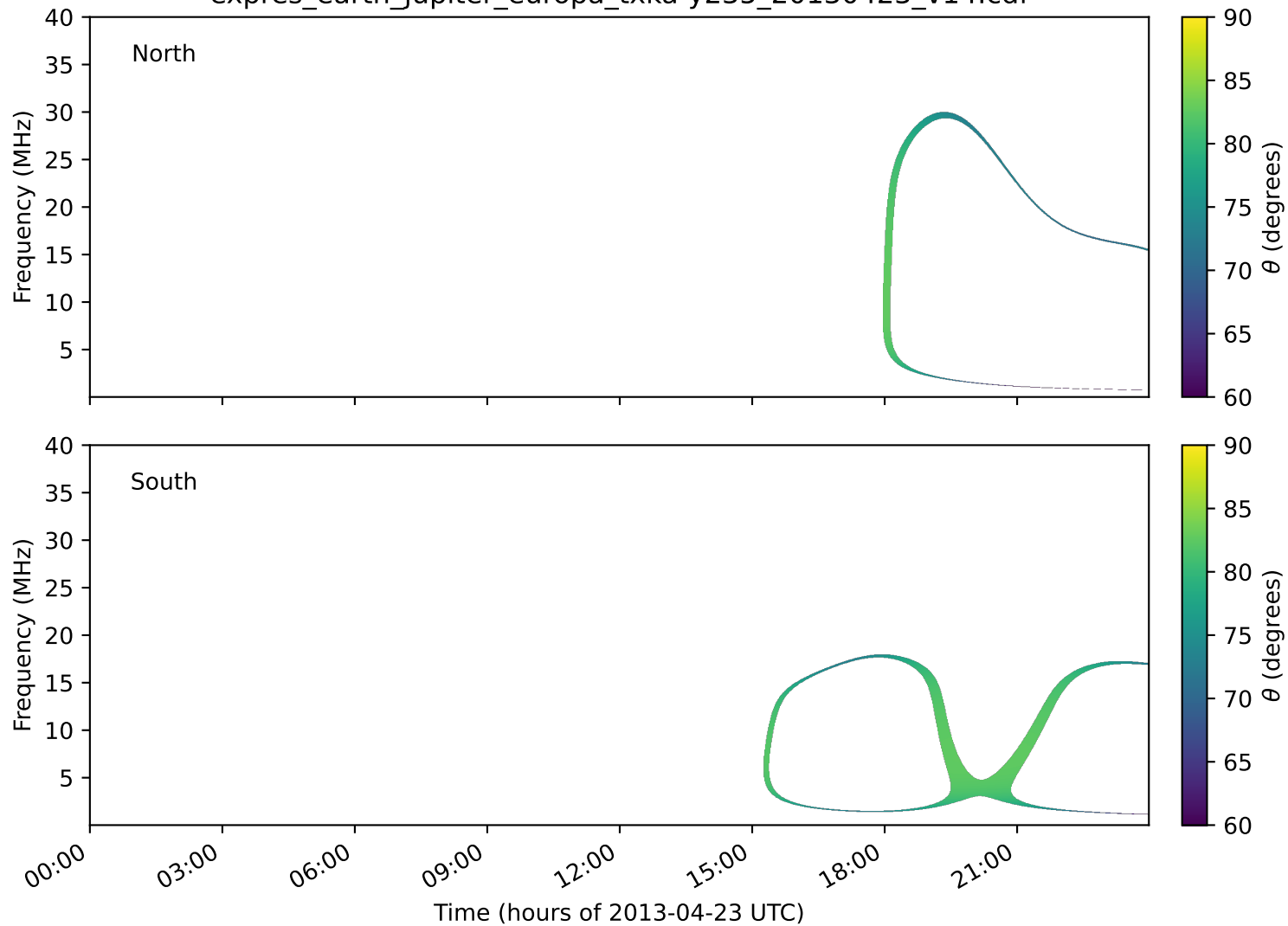
expres_earth_jupiter_europa_txka-y235_20130423_v14.cdf
