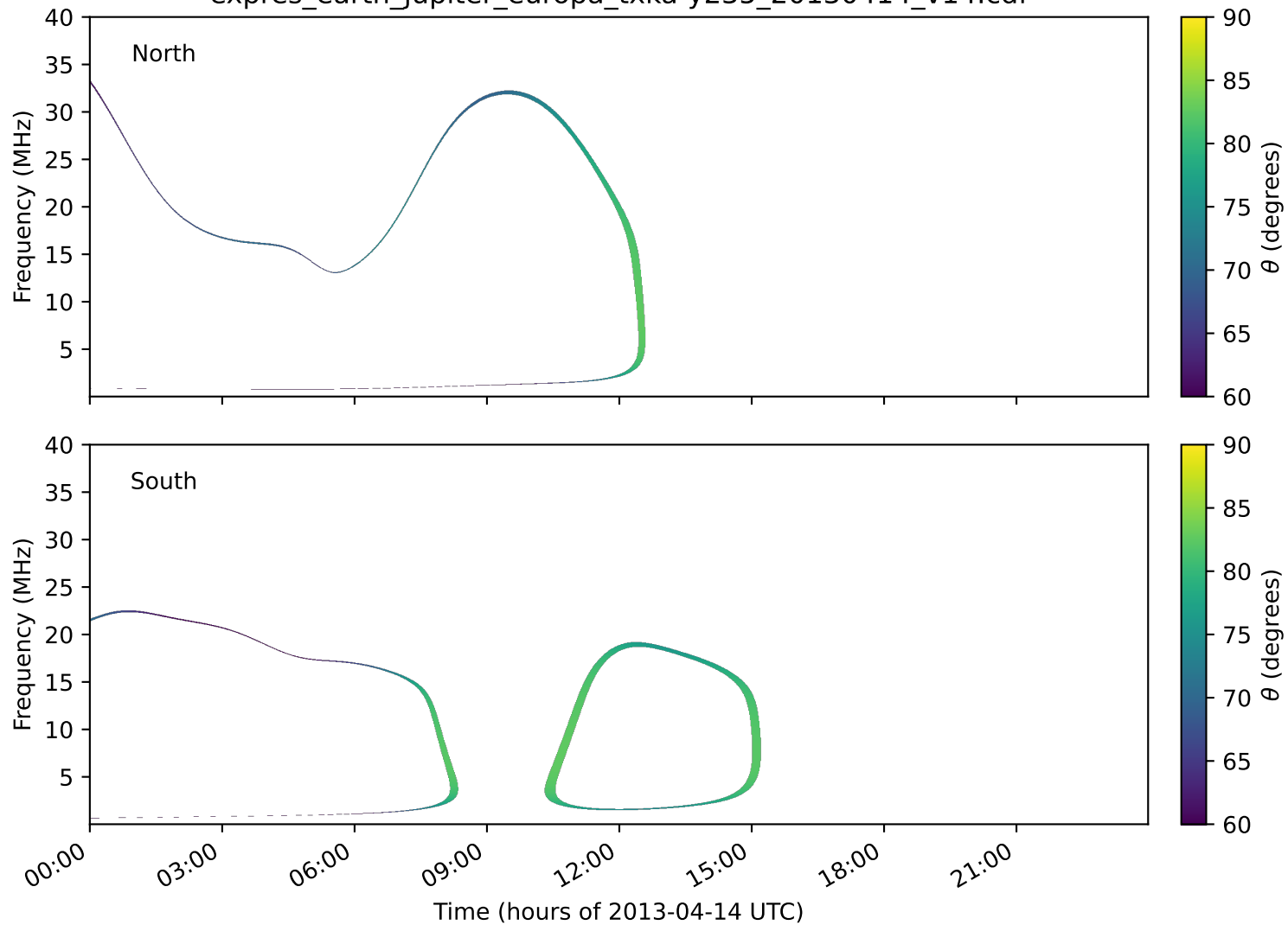
expres_earth_jupiter_europa_txka-y235_20130414_v14.cdf
