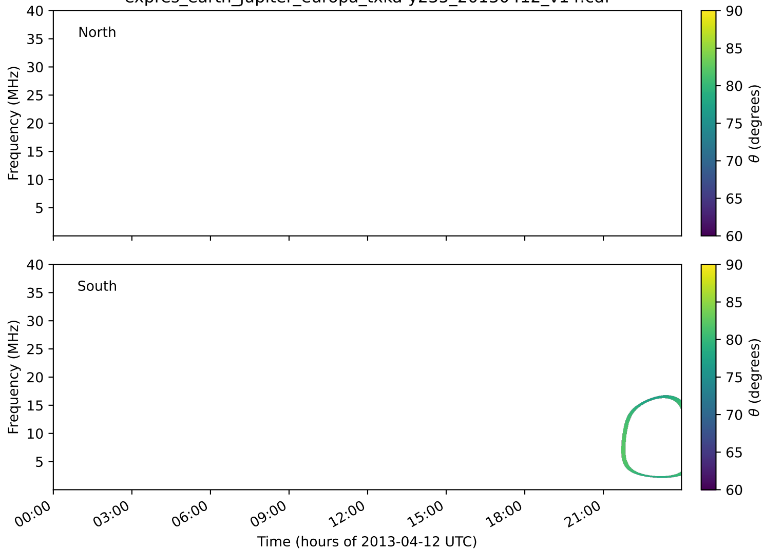
expres_earth_jupiter_europa_txka-y235_20130412_v14.cdf
