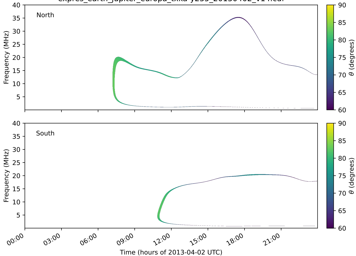
expres_earth_jupiter_europa_txka-y235_20130402_v14.cdf
