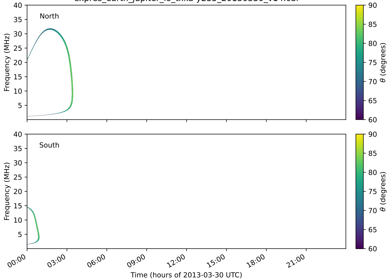
expres_earth_jupiter_io_txka-y235_20130330_v14.cdf
