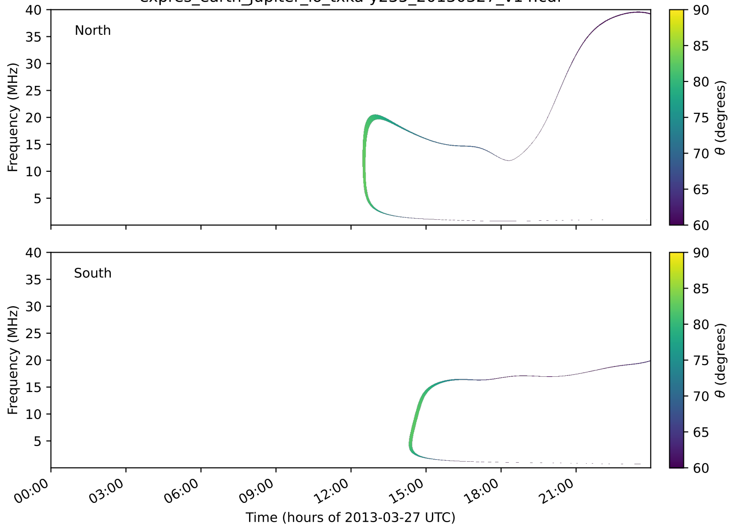
expres_earth_jupiter_io_txka-y235_20130327_v14.cdf
