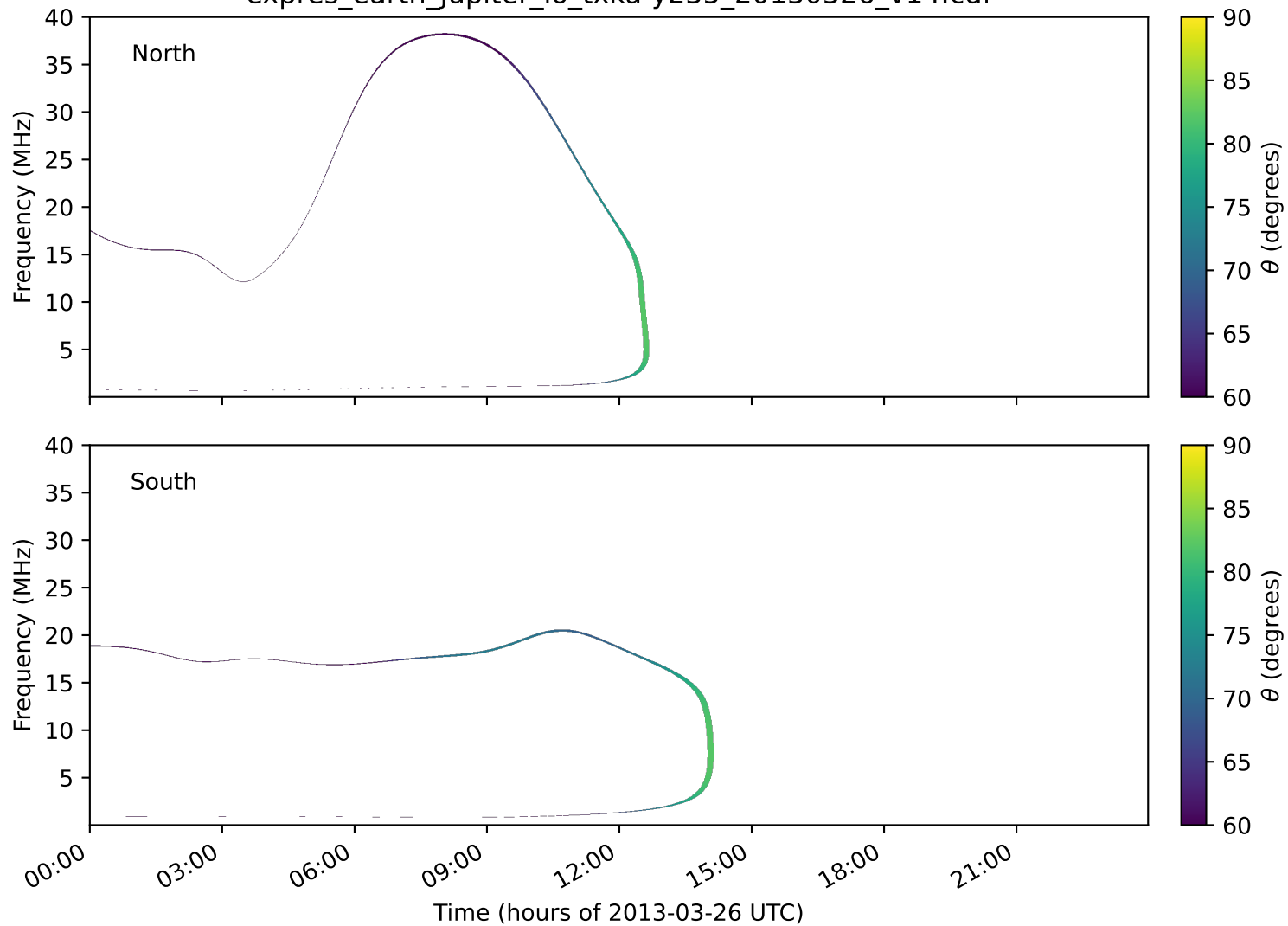
expres_earth_jupiter_io_txka-y235_20130326_v14.cdf
