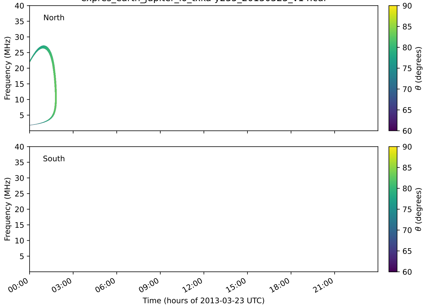
expres_earth_jupiter_io_txka-y235_20130323_v14.cdf
