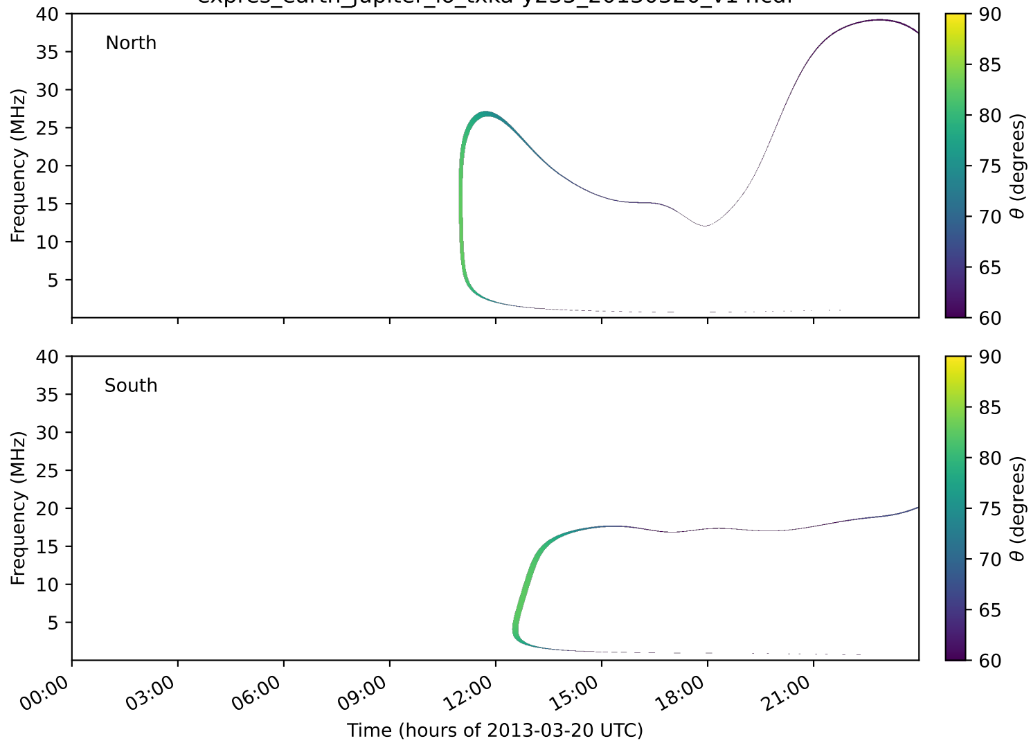
expres_earth_jupiter_io_txka-y235_20130320_v14.cdf
