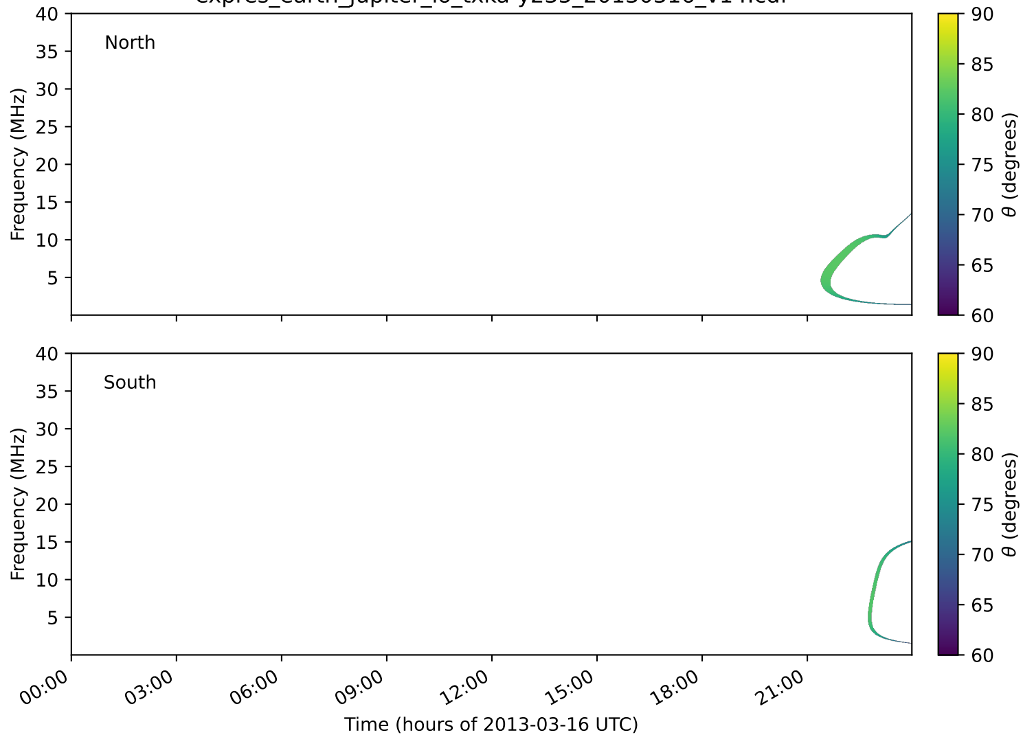
expres_earth_jupiter_io_txka-y235_20130316_v14.cdf
