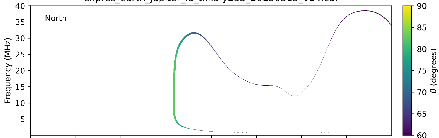
expres_earth_jupiter_io_txka-y235_20130313_v14.cdf
