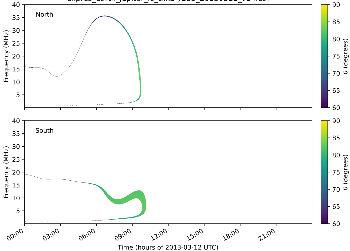
expres_earth_jupiter_io_txka-y235_20130312_v14.cdf
