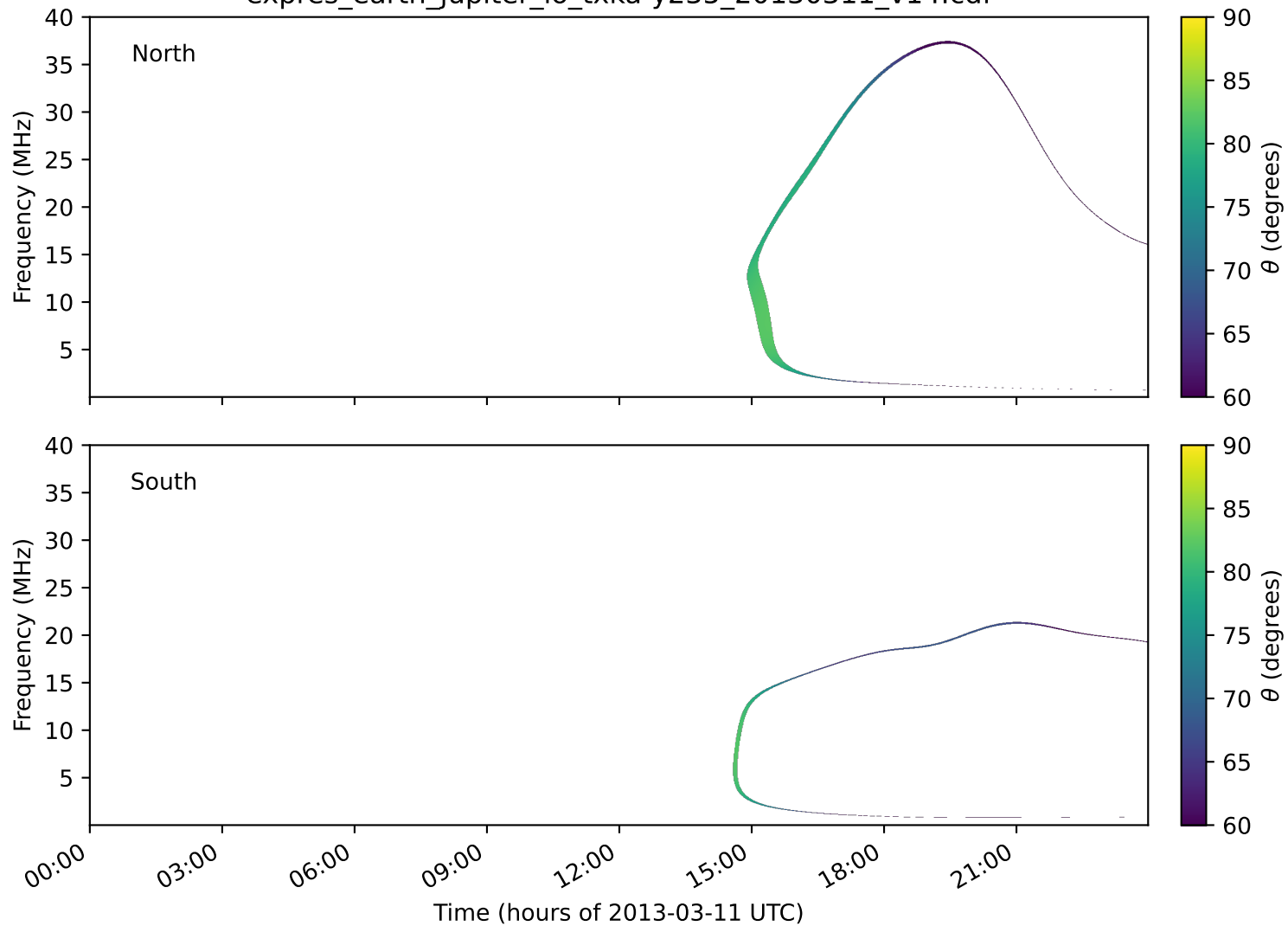
expres_earth_jupiter_io_txka-y235_20130311_v14.cdf
