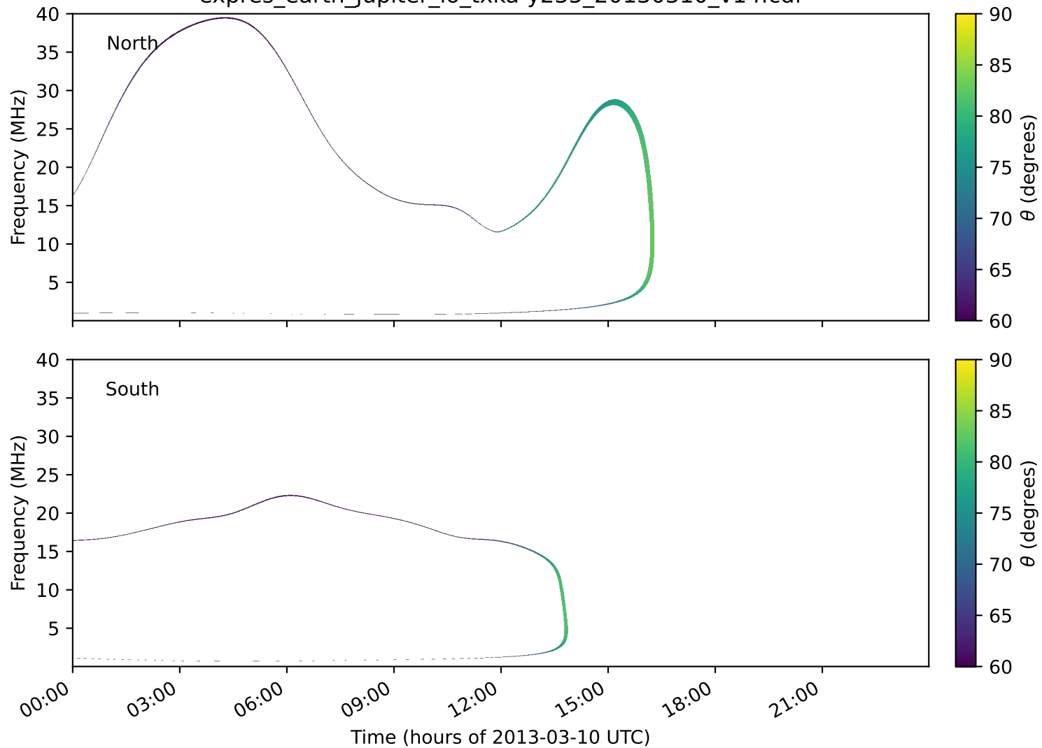
expres_earth_jupiter_io_txka-y235_20130310_v14.cdf
