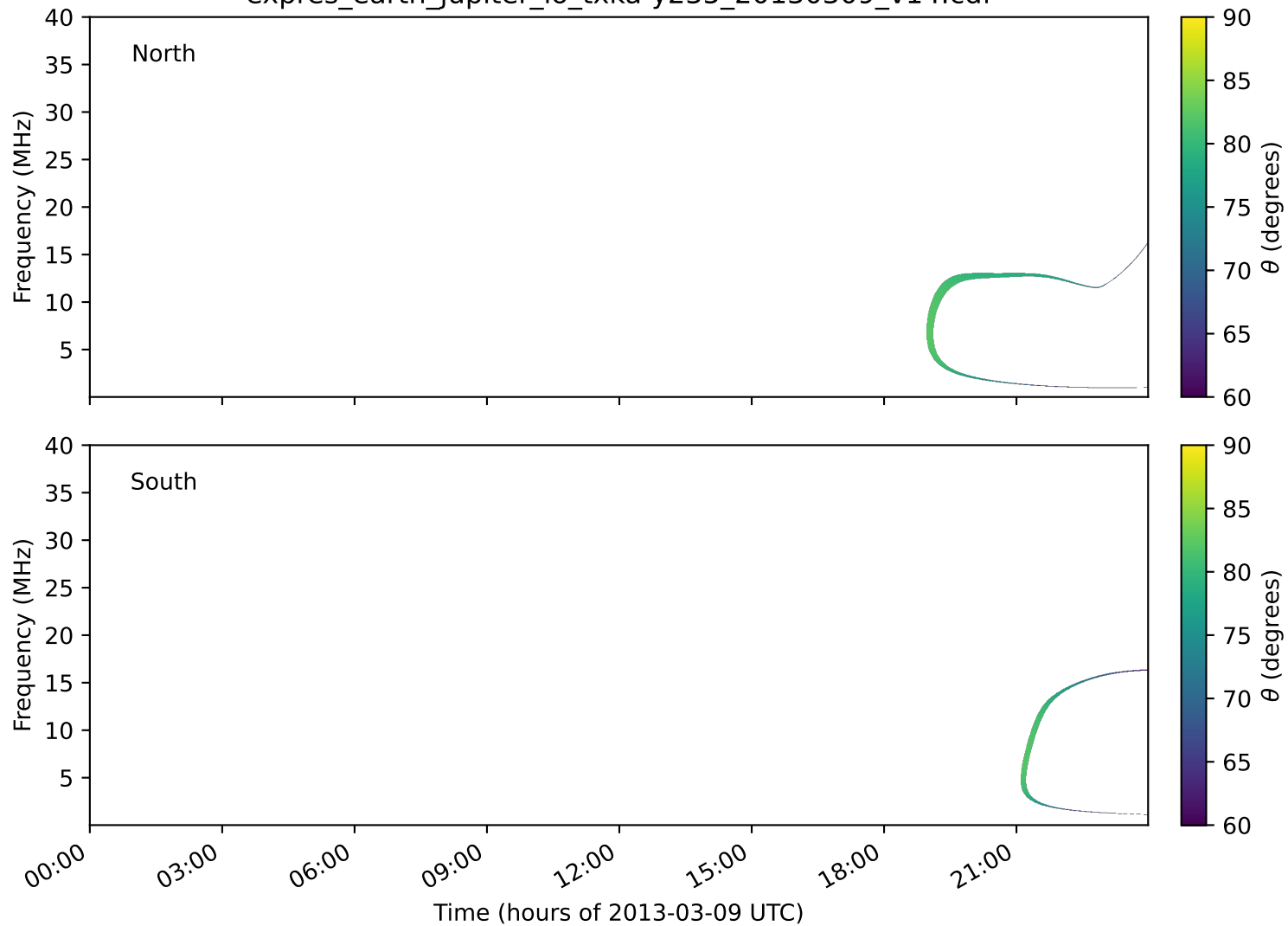
expres_earth_jupiter_io_txka-y235_20130309_v14.cdf
