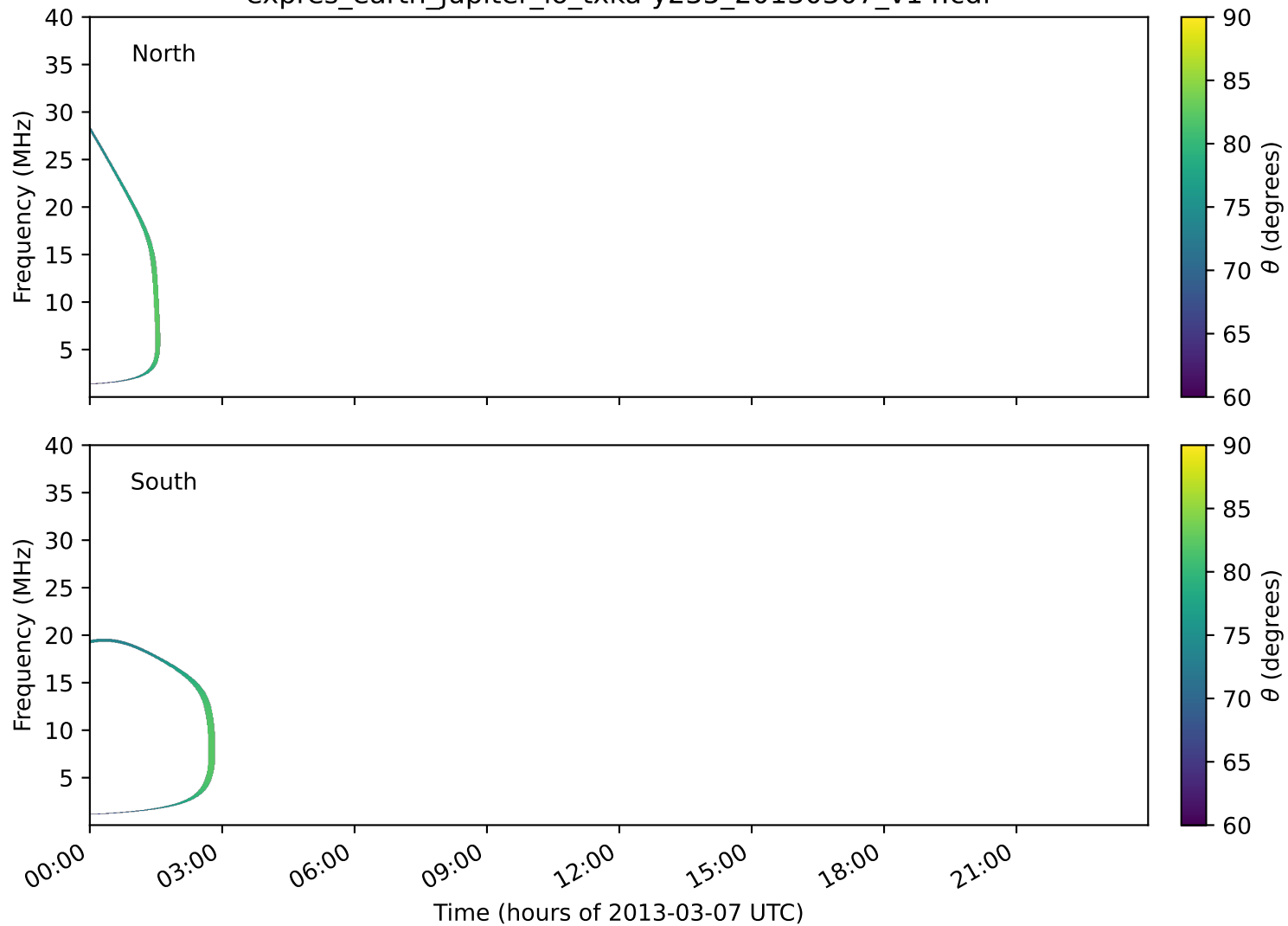
expres_earth_jupiter_io_txka-y235_20130307_v14.cdf
