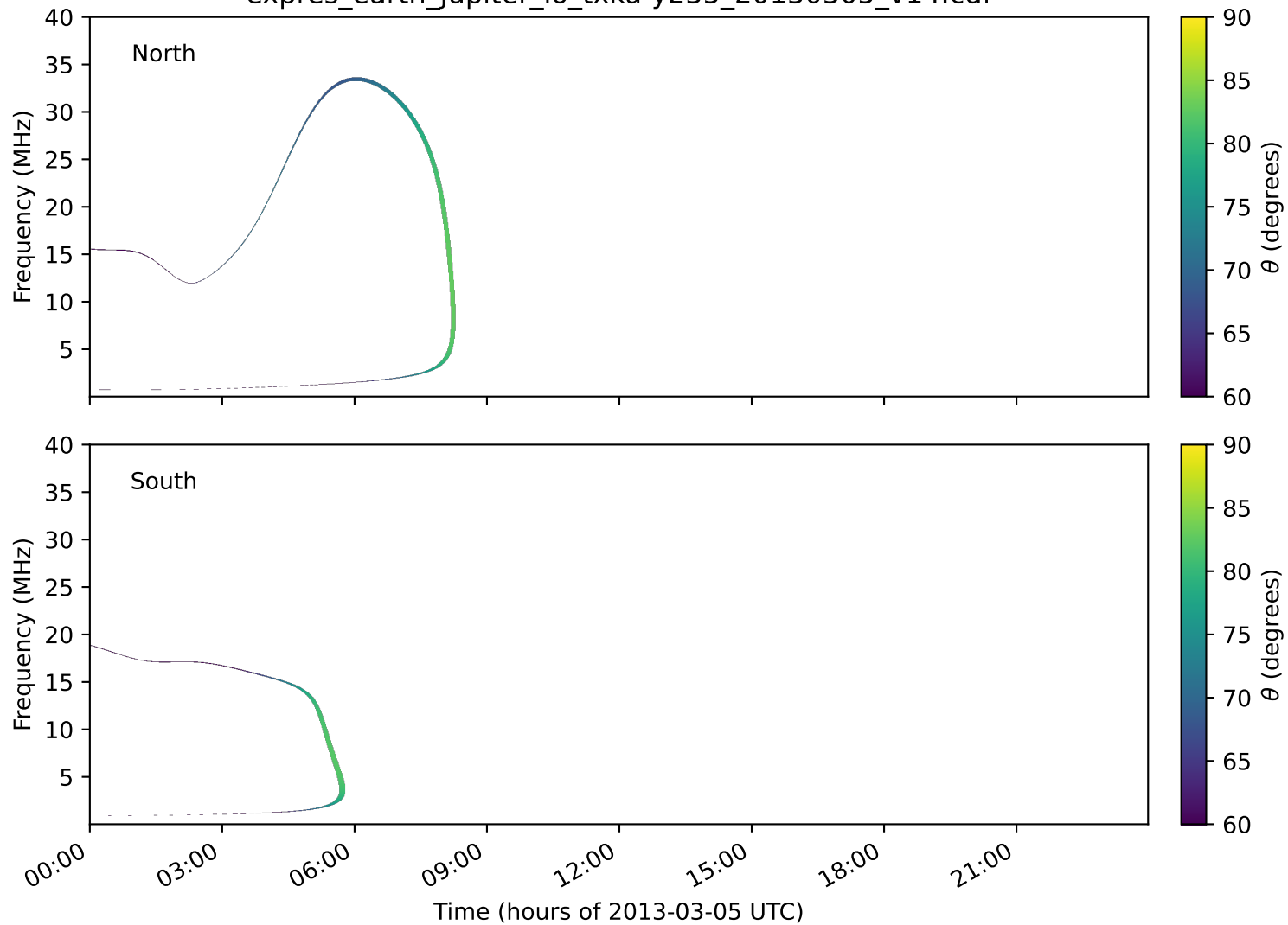
expres_earth_jupiter_io_txka-y235_20130305_v14.cdf
