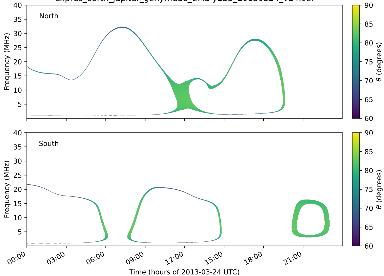
expres_earth_jupiter_ganymede_txka-y235_20130324_v14.cdf
