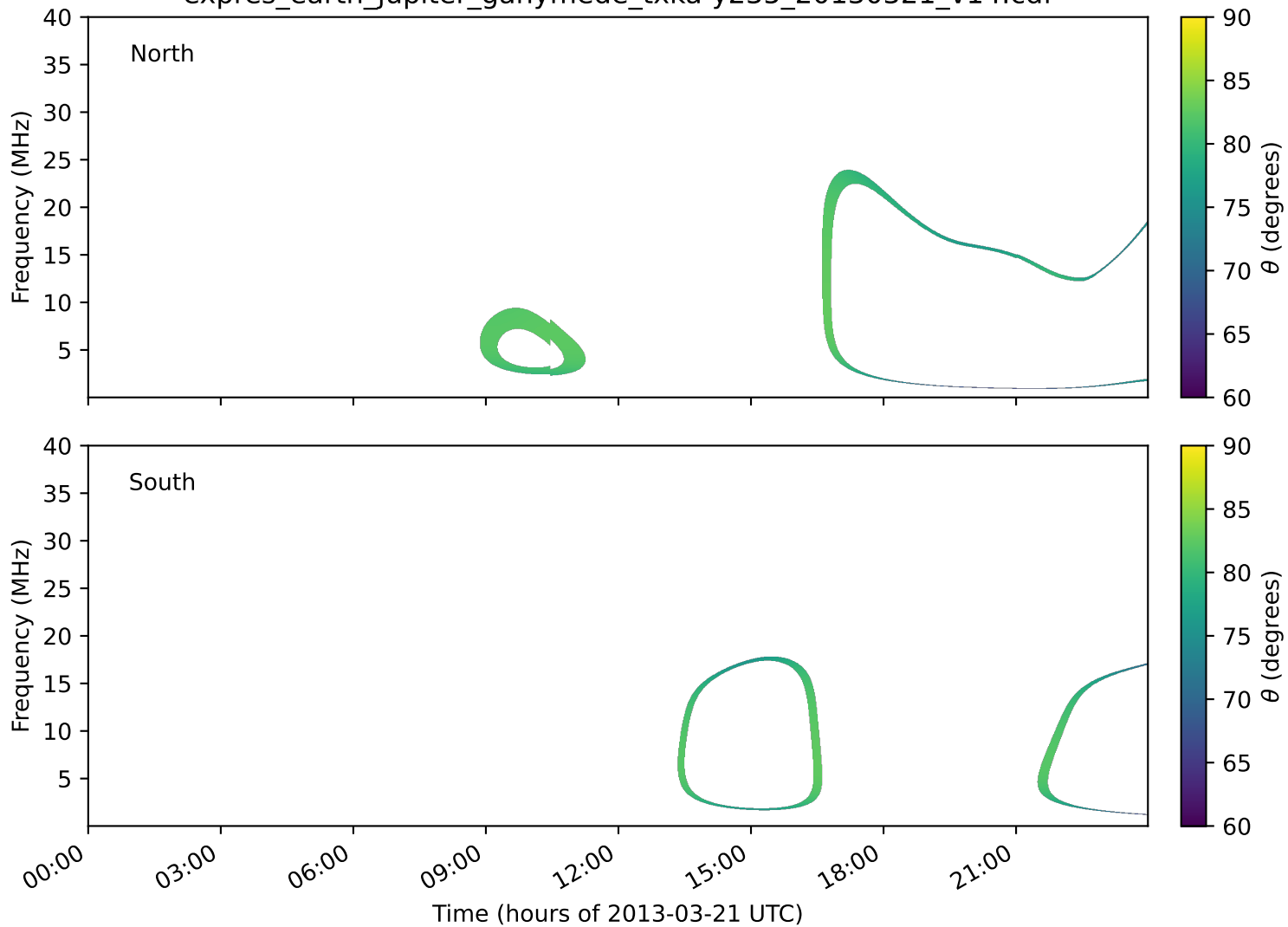
expres_earth_jupiter_ganymede_txka-y235_20130321_v14.cdf
